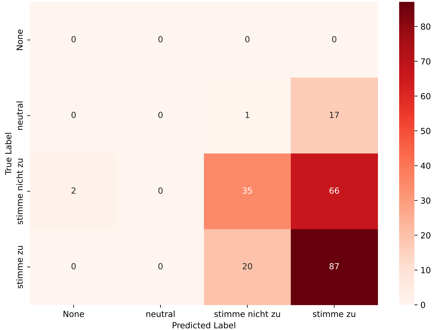
Confusion Matrix - Llama 3, temp: 0.7
